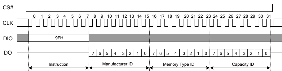
Figure 7.15 Read JEDEC ID instruction Sequence Diagram
