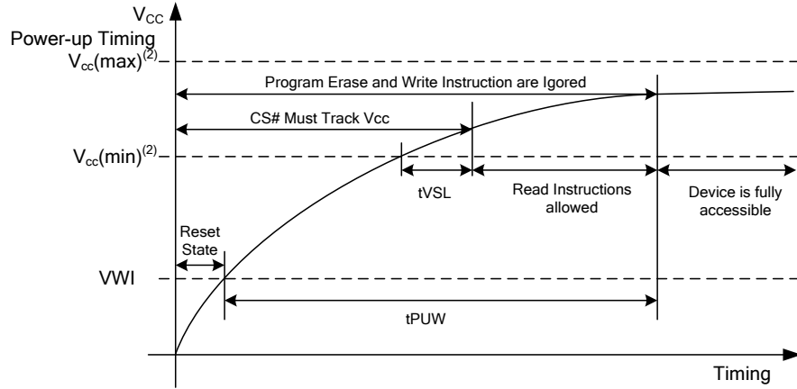
Figure 8.1 Power-up Timing
