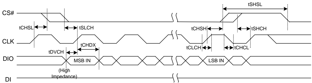
Figure 8.4 Input Timing
