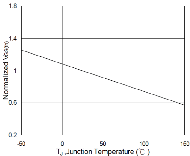
Figure 5: Normalized VGS (v.s Tj)
