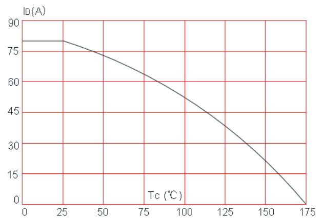
Figure 11: Maximum Continuous Drain Current vs. Temperature
