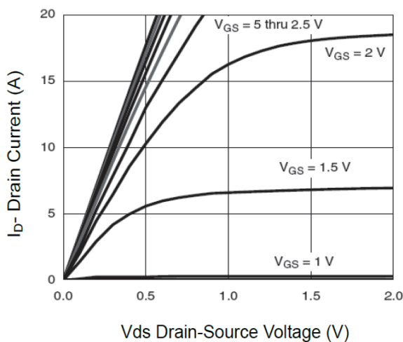
Figure 5: Output Characteristics
