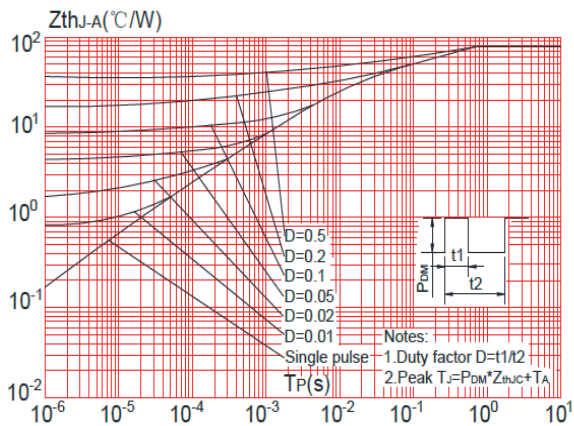
Figure 11: Maximum Effective Transient Thermal Impedance vs. Junction to Ambient
