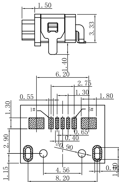
RECOMMENDED PCB LAYOUT (TOP VIEW)
