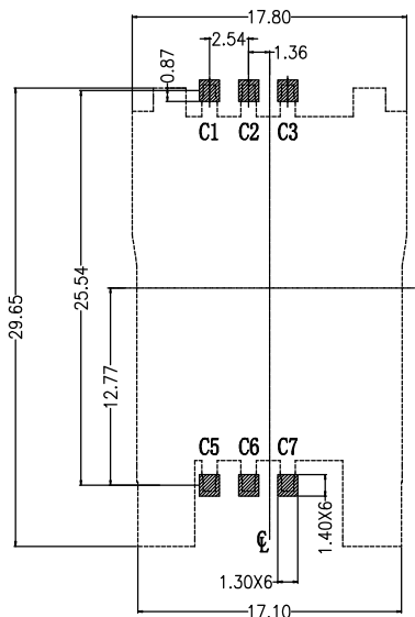
RECOMMENDED PCB LAYOUT TOLERANCE: ±0.05
