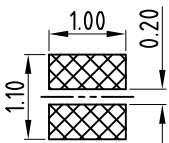
METAL MASK T=0.08 TOLERANCE:±0.05MM (FOR REFERENCE ONLY)
