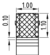
RECOMMENDED PCB LAYOUT TOLERANCE:±0.05MM (FOR REFERENCE ONLY)
