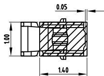
RECOMMENDED PCB LAYOUT TOLERANCE ±0.05 (焊盘推荐图)
