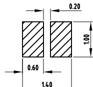
METAL MASK T=0.10 TOLERANCE ±0.05 (钢网推荐图)
