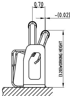
STATED AT COMPRESSION (FOR REFERENCE ONLY)
