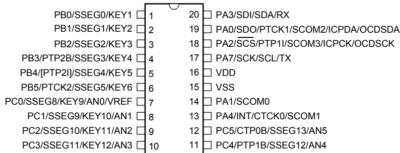
BS86B12A-3/BS86BV12A 20 SOP-A
