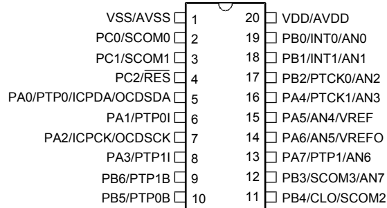
HT66F004/HT66V004 20 SOP-A/SSOP-A/DIP-A
