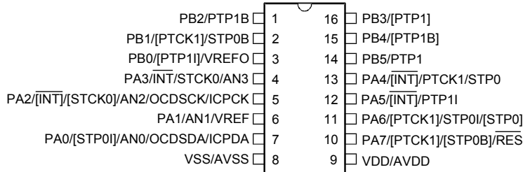
HT66F003/HT66V003 16 NSOP-A
