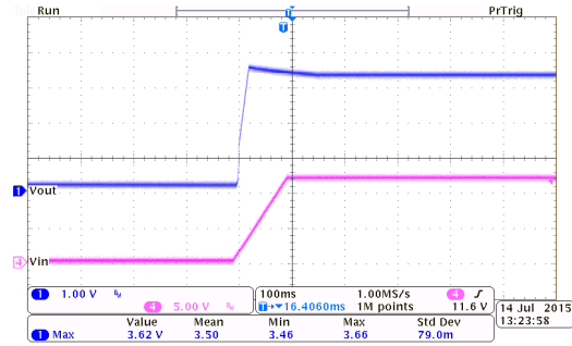
Power On Response: HT7333-2 ( I_{OUT}=0mA , T_{RISE}=100ms )
