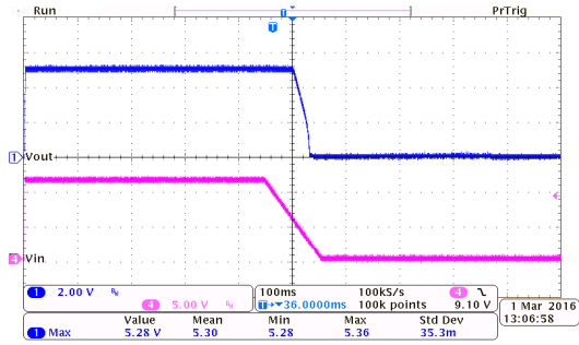
掉电响应: HT7350-7 ( I_{OUT}=250mA , T_{FALL}=100ms )
