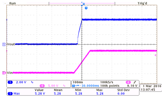
上电响应: HT7350-7 ( I_{OUT}=250mA , T_{RISE}=100ms )
