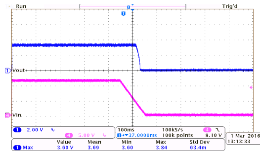
掉电响应: HT7333-7 ( I_{OUT}=250mA , T_{FALL}=100ms )
