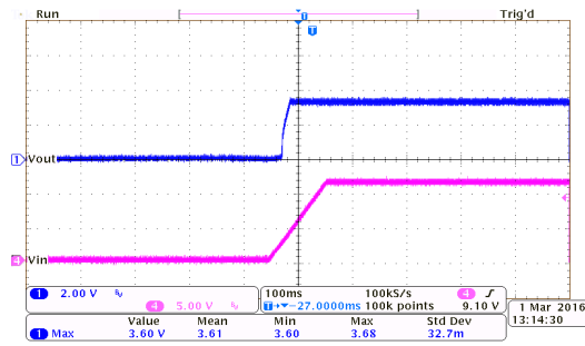
上电响应: HT7333-7 ( I_{OUT}=250mA , T_{RISE}=100ms )
