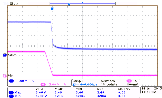
Power Off Response: HT7333-1 ( I_{OUT}=0mA , T_{FALL}=0.1ms )
