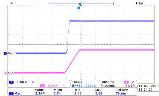
Power On Response: HT7333-1 ( I_{OUT}=250mA , T_{RISE}=100ms )
