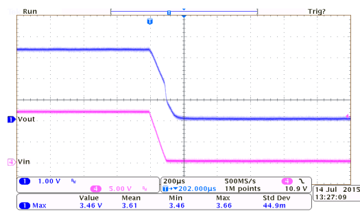
Power Off Response: HT7333-1 ( I_{OUT}=250mA , T_{FALL}=0.1ms )
