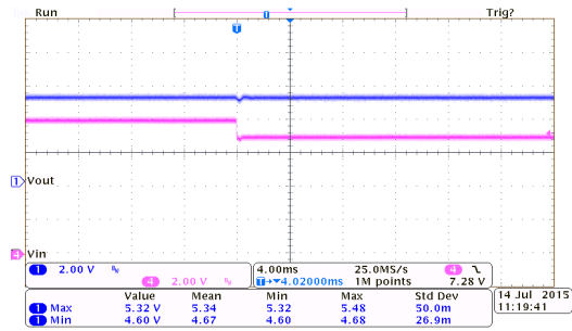
Line Transient Response: HT7350-1 ( I_{OUT}=10mA )
