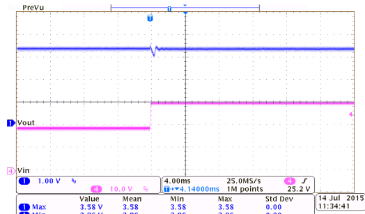
Line Transient Response: HT7333-2 ( I_{OUT}=10mA )
