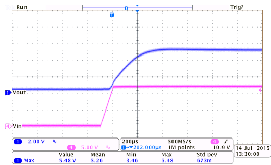
Power On Response: HT7350-2 ( I_{OUT}=0mA , T_{RISE}=0.1ms )
