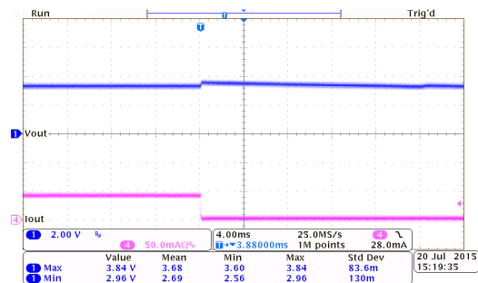
Load Transient Response: HT7333-3 ( V_{IN}=5.3V , I_{OUT}=40mA to 0mA )
