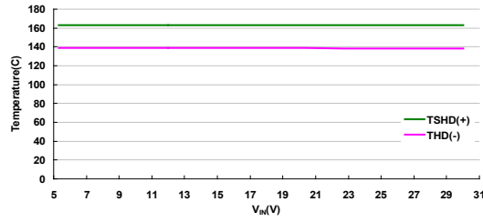
TSHD VS V_{IN}
