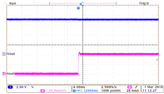
负载瞬态响应： HT7350-7 ( V_{IN}=7.0V , I_{OUT}=0mA to 40mA )
