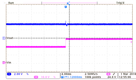
线性瞬态响应: HT7333-7 ( I_{OUT}=10mA )
