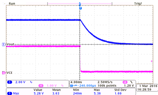
掉电响应: HT7350-7 ( I_{OUT}=0mA, V_{CE}=2.7V to 0V)
