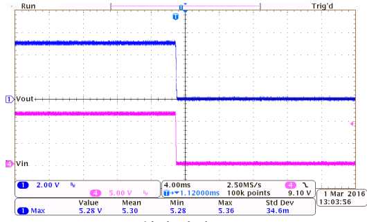
掉电响应: HT7350-7 ( I_{OUT}=250mA , T_{FALL}=0.1ms )
