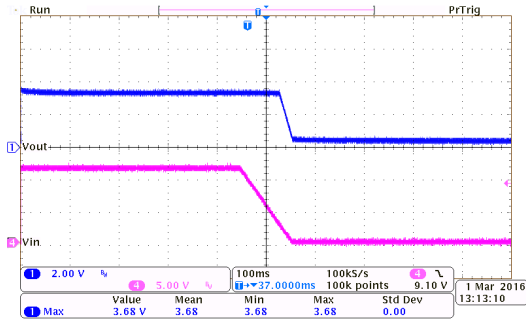
掉电响应: HT7333-7 ( I_{OUT}=0mA , T_{FALL}=100ms )
