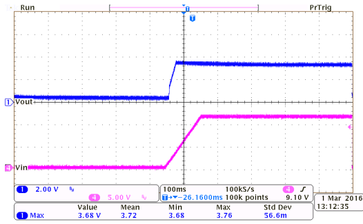
上电响应: HT7333-7 ( I_{OUT}=0mA , T_{RISE}=100ms )
