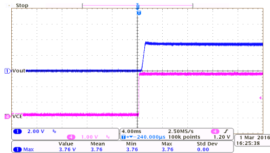
上电响应: HT7333-7 ( I_{OUT}=0mA, V_{CE}=0V to 2.7V)
