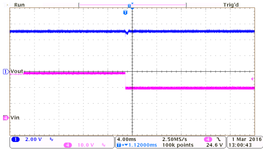
线性瞬态响应: HT7350-7 ( I_{OUT}=10mA )
