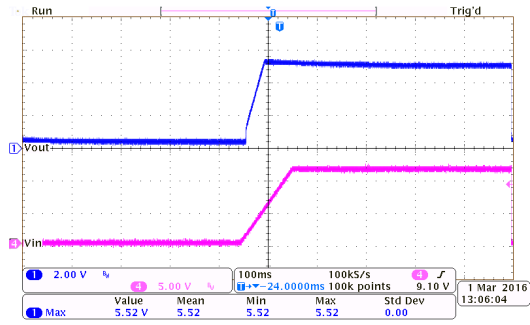
上电响应: HT7350-7 ( I_{OUT}=0mA , T_{RISE}=100ms )
