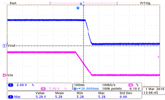
掉电响应: HT7350-7 ( I_{OUT}=0mA , T_{FALL}=100ms )
