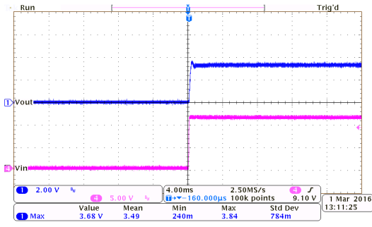
上电响应: HT7333-7 ( I_{OUT}=250mA , T_{RISE}=0.1ms )
