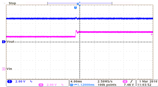
线性瞬态响应：HT7350-7 ( I_{OUT}=10mA )
