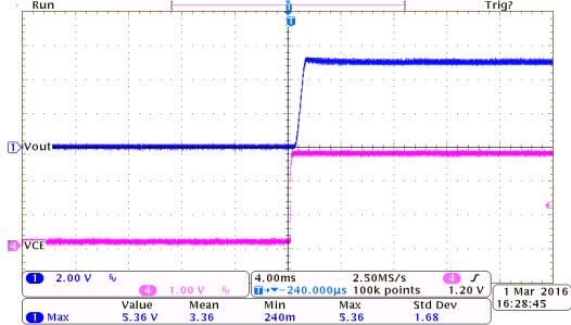
上电响应: HT7350-7 ( I_{OUT}=0mA, V_{CE}=0V to 2.7V)
