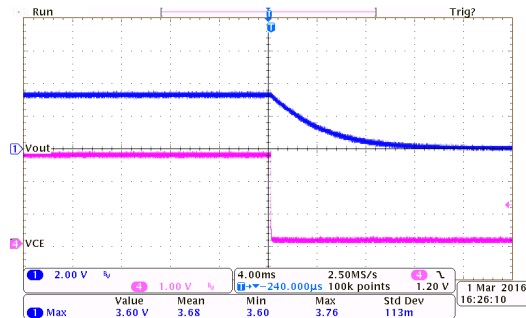
掉电响应: HT7333-7 ( I_{OUT}=0mA, V_{CE}=2.7V to 0V)
