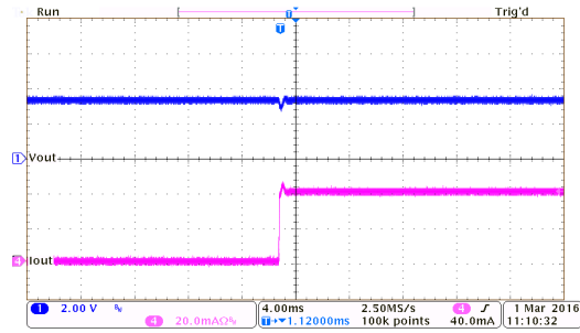
负载瞬态响应： HT7333-7 ( V_{IN}=5.3V , I_{OUT}=0mA to 40mA )
