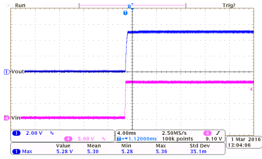
上电响应: HT7350-7 ( I_{OUT}=250mA , T_{RISE}=0.1ms )
