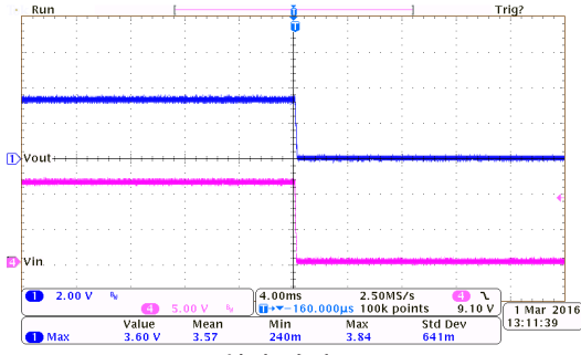
掉电响应: HT7333-7 ( I_{OUT}=250mA , T_{FALL}=0.1ms )
