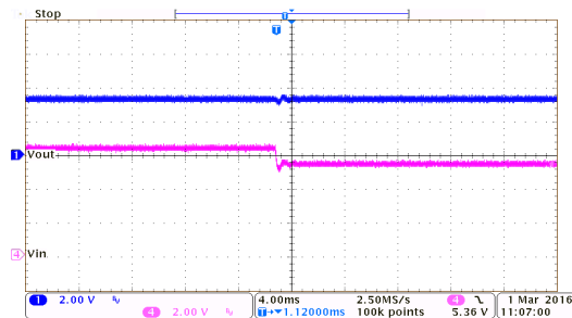
线性瞬态响应：HT7333-7 ( I_{OUT}=10mA )
