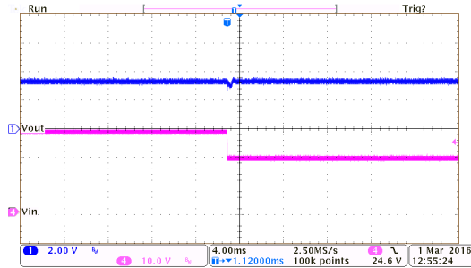
线性瞬态响应: HT7333-7 ( I_{OUT}=10mA )
