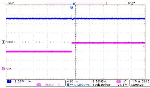
线性瞬态响应: HT7350-7 ( I_{OUT}=10mA )
