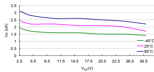
I SS vs V CE : HT75C0-7 (I OUT =0mA)
