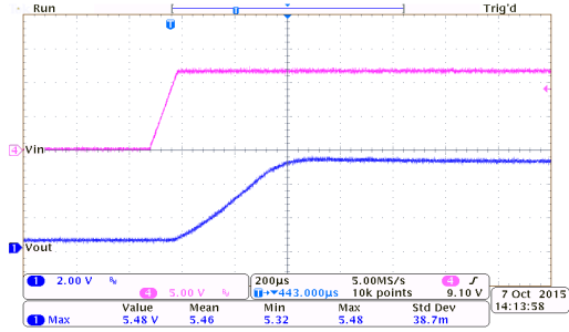
Power On Response: HT7550-7 ( I_{OUT}=0mA , T_{RISE}=0.1ms )
