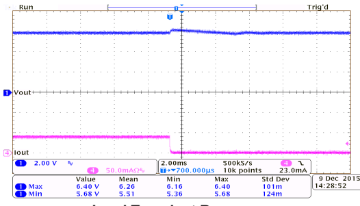
Load Transient Response: HT7560-7 ( V_{IN}=8.0V , I_{OUT}=40mA to 0mA )
