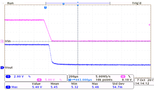
Power Off Response: HT7550-7 ( I_{OUT}=0mA , T_{FALL}=0.1ms )
