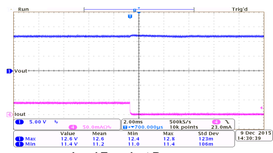
Load Transient Response: HT75C0-7 ( V_{IN}=14V , I_{OUT}=40mA to 0mA )
