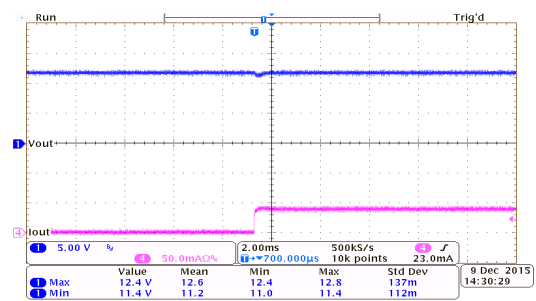
Load Transient Response: HT75C0-7 ( V_{IN}=14V , I_{OUT}=0mA to 40mA )
