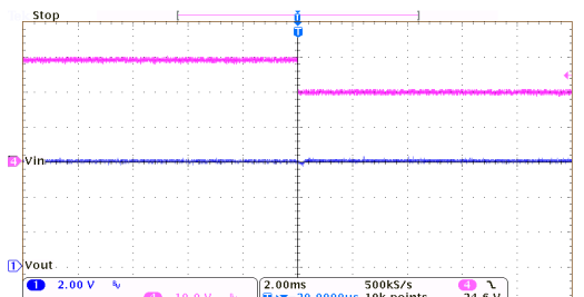
Line Transient Response: HT7560-7 ( I_{OUT}=10mA )
