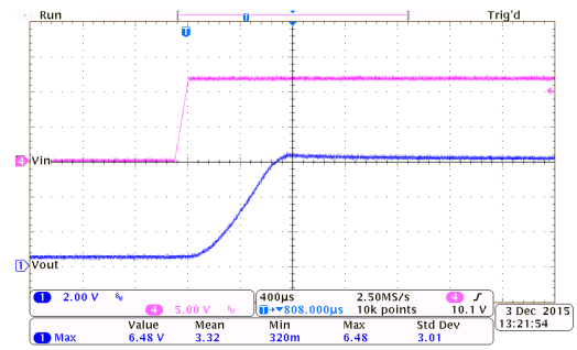
Power On Response: HT7560-7 ( I_{OUT}=0mA , T_{RISE}=0.1ms )
