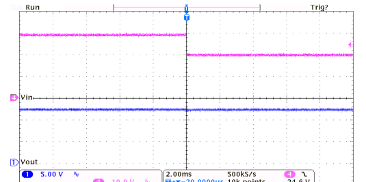
Line Transient Response: HT75C0-7 ( I_{OUT}=10mA )
