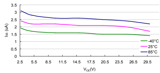
I_{SS} vs V_{CE} : HT75C0-7 ( I_{OUT}=0mA )
