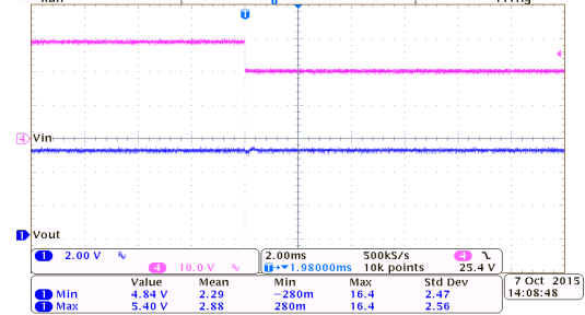
Line Transient Response: HT7550-7 ( I_{OUT}=10mA )
