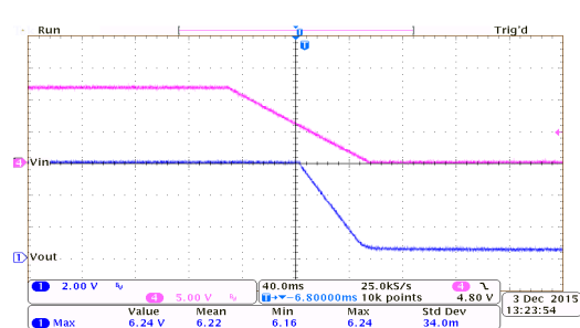
Power Off Response: HT7560-7 ( I_{OUT}=150mA , T_{FALL}=100ms )
