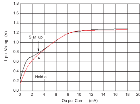
HT7750 Start-Up & Hold-On Voltage
