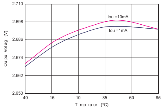
HT7727 Temperature v.s Output Voltage
