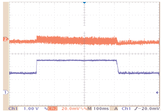
HT7733 Line Transient Response (L=100µH, C OUT =100µF)
