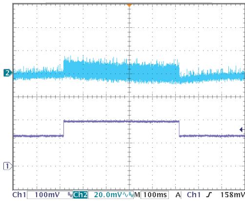
HT7722 Line Transient Response (L=100µH, C OUT =100µF)
