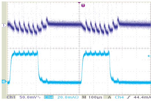
HT7750 Load Transient Response (L=100µH, C OUT =100µF, V IN =3V)
