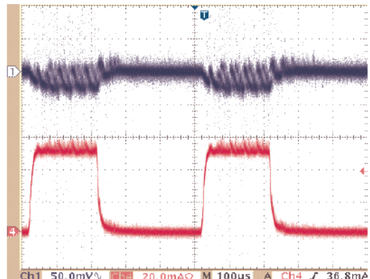
HT7737 Load Transient Response (L=100 \mu H, C OUT =100 \mu F, V IN =2.22V)
