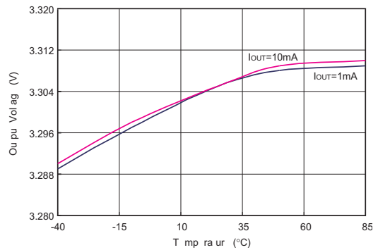
HT7733 Temperature v.s Output Voltage
