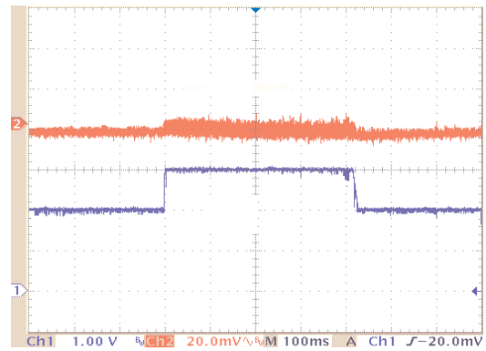
HT7750 Line Transient Response (L=100µH, C OUT =100µF)
