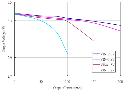
Fig 17. HT7733S Output Voltage vs. Output Current
