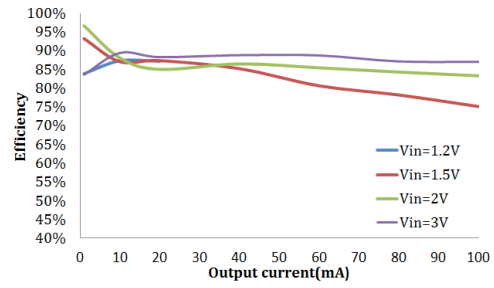
HT7750B Efficiency vs. Output Current
