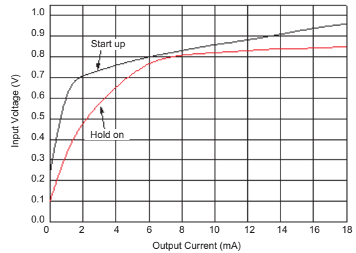
HT7727 Start-Up & Hold-On Voltage
