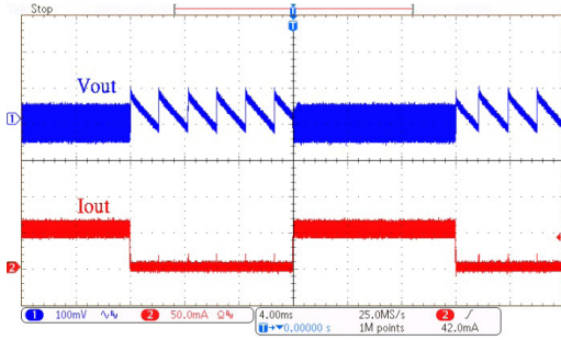
HT7733B Load Transient (1mA to 50mA)
