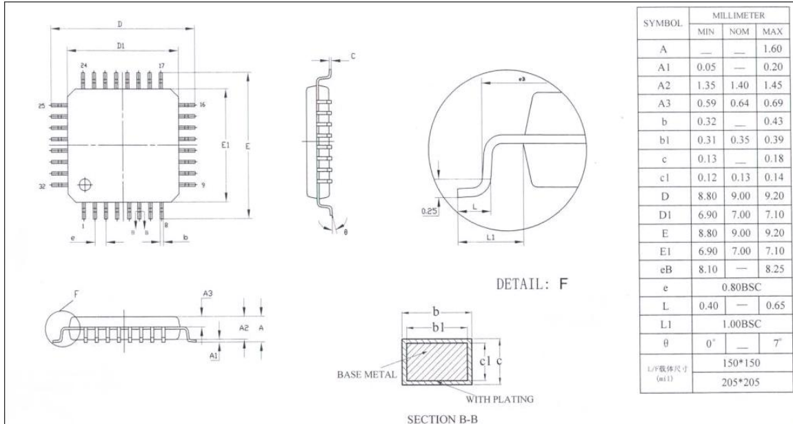
Figure 24-1 LQFP32 封装尺寸
