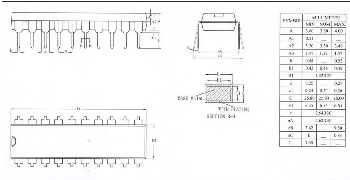
Figure 24-3 DIP20 封装尺寸
