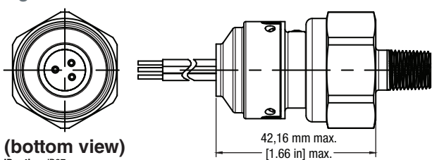
Figure 24. Wire out
