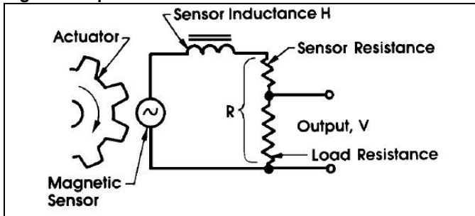
Figure 8. Equivalent Circuit
