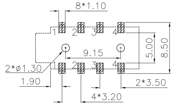
RECOMMEND PCB LAYOUT(±0.05)
