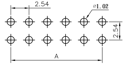
RECOMMEND P.C.B LAYOUT PCB TOLERANCE: ±0.05 (TOP VIEW)
