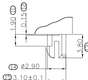
DETAIL "X" SCALE 2:1
