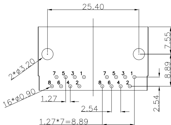
RECOMMENDED PCB LAYOUT TOP VIEW(TOL:±0.05)
