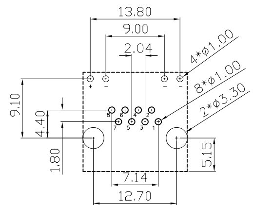
RECOMMENDER P.C.B.LAYOUT TOP VIEW (COMPONENT SIDE TOLERANCE±0.05)
