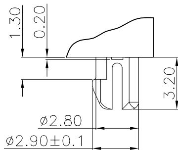
DETAIL "X" SCALE 2:1
