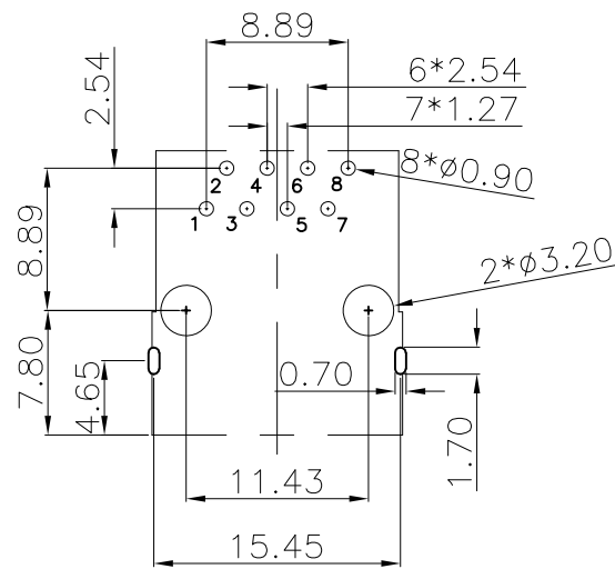
RECOMMENDED PCB LAYOUT TOP VIEW(TOL:±0.05)
