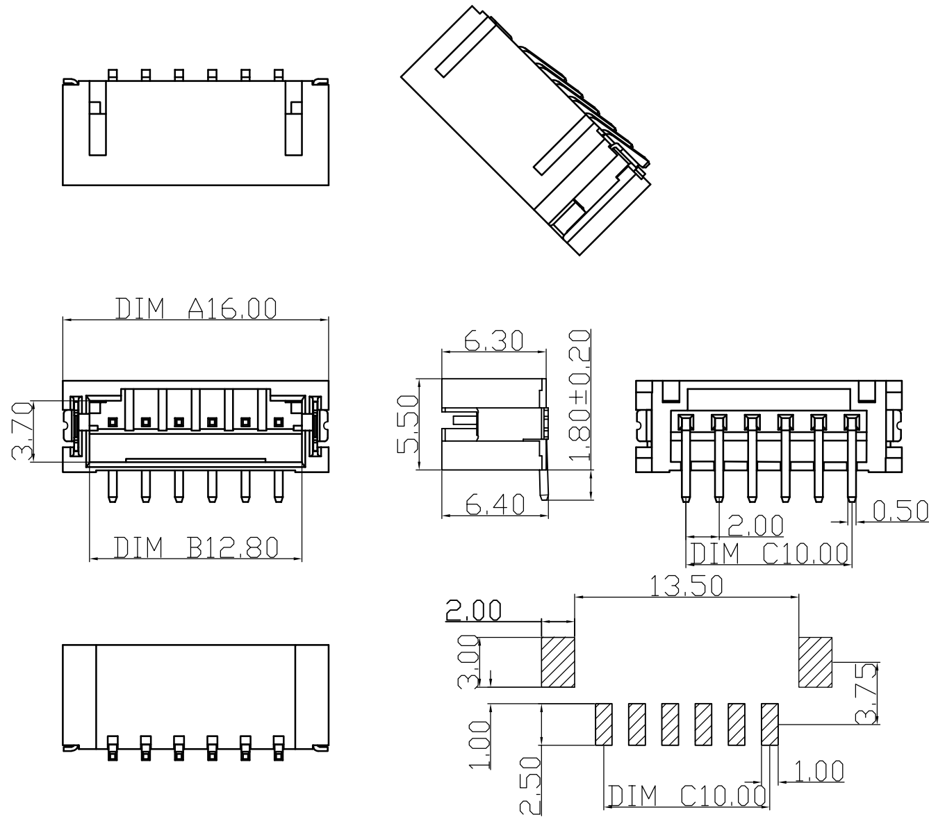
RECOMMENDER P.C.B. LAYOUT TOP VIEW
