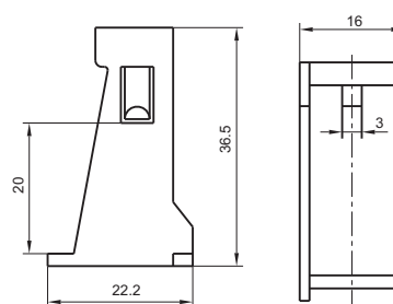
140F-H1(Plastic retainer)
