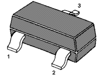
Marking Code: C3 SOT-23 Plastic Package
