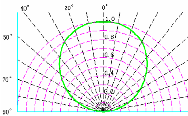
Typical optical characteristics curves 光电特性曲线 Curves of beam angle and relative brightness 角度图
