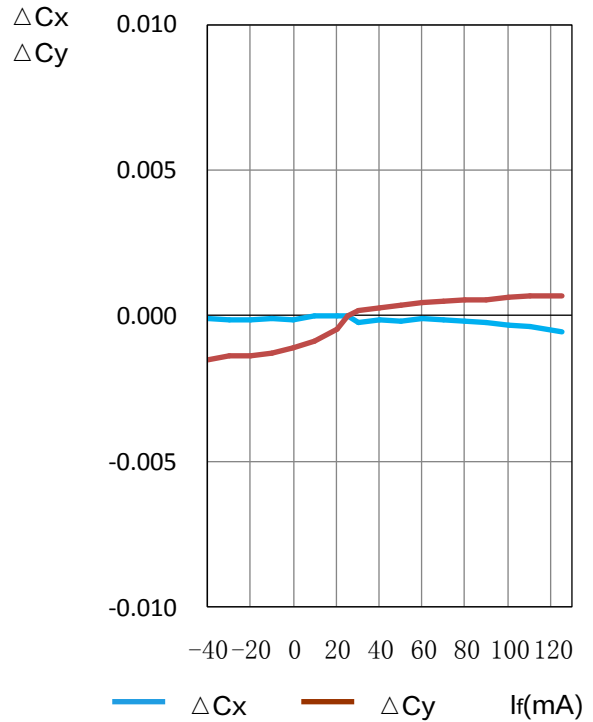
色坐标数据表/Chromaticity coordinate shift \Delta C_x, \Delta C_y = f(I_f); I_f = 20\text{mA}
