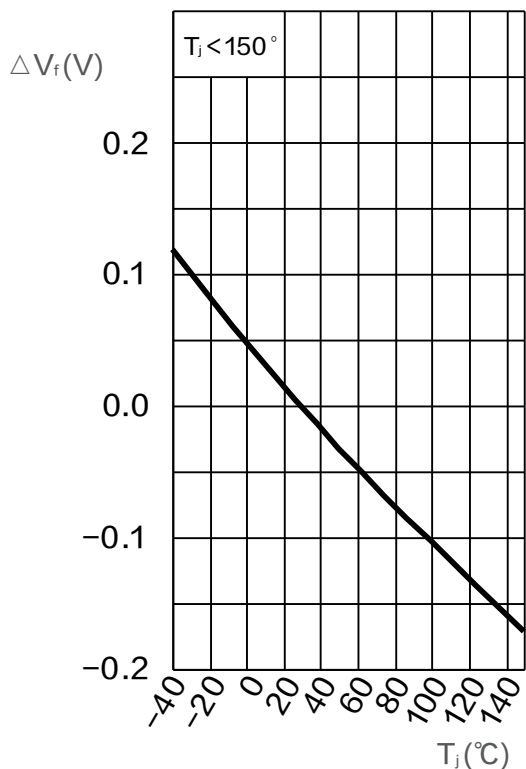
相对正向电压 / Relative Forward Voltage \Delta V_f = V_f - V_f(25^\circ C) = f(T_j); I_f = 1000 mA
