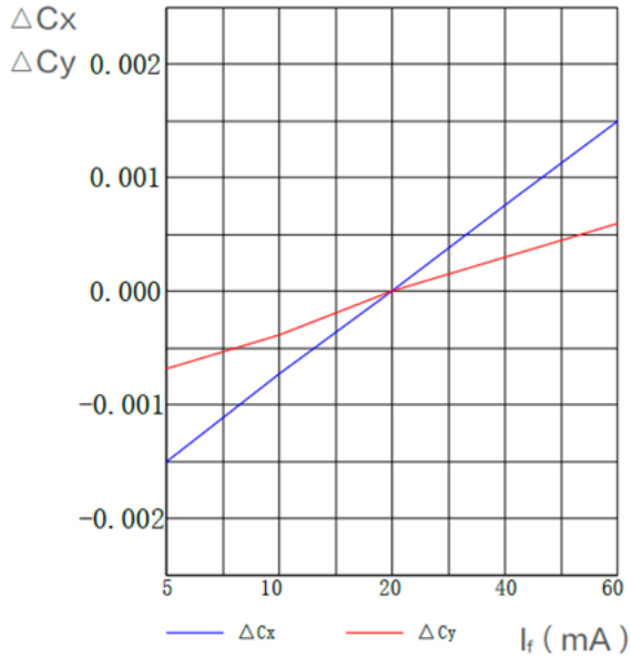
色坐标数据表/Chromaticity coordinate shift \Delta Cx, \Delta Cy = f(I_f); T_s = 25^\circ C
