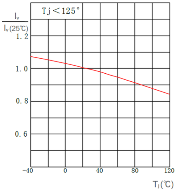
相对发光强度 / Relative Luminous Intensity I_v / I_v(25^\circ C) = f(T_j); I_f = 20 mA
