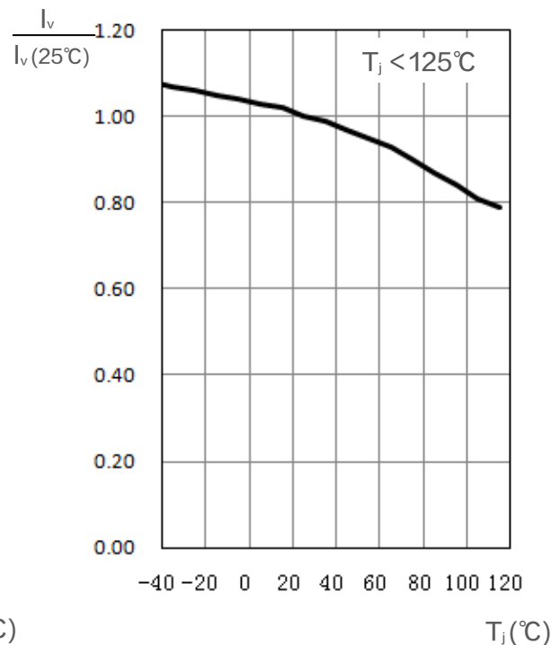
相对发光强度 / Relative Luminous Intensity I_v / I_v(25^\circ C) = f(T_j); I_f = 50 mA
