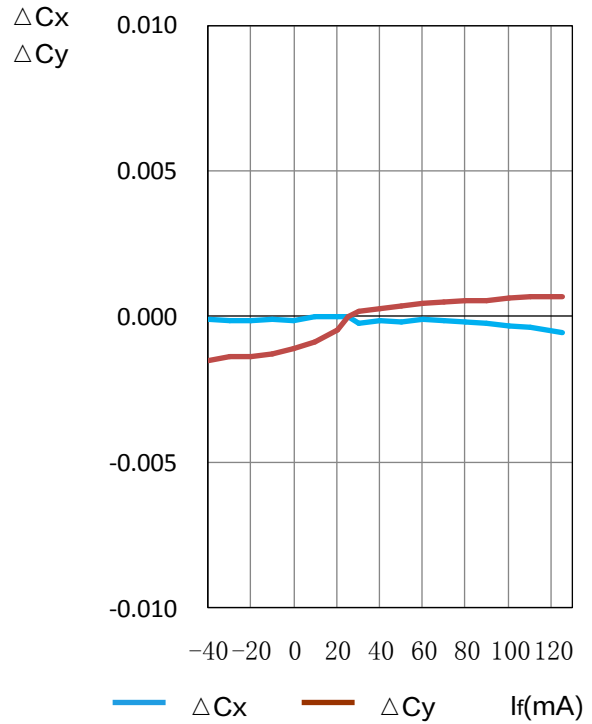
色坐标数据表/Chromaticity coordinate shift \Delta Cx, \Delta Cy = f(I_f); I_f = 50 mA
