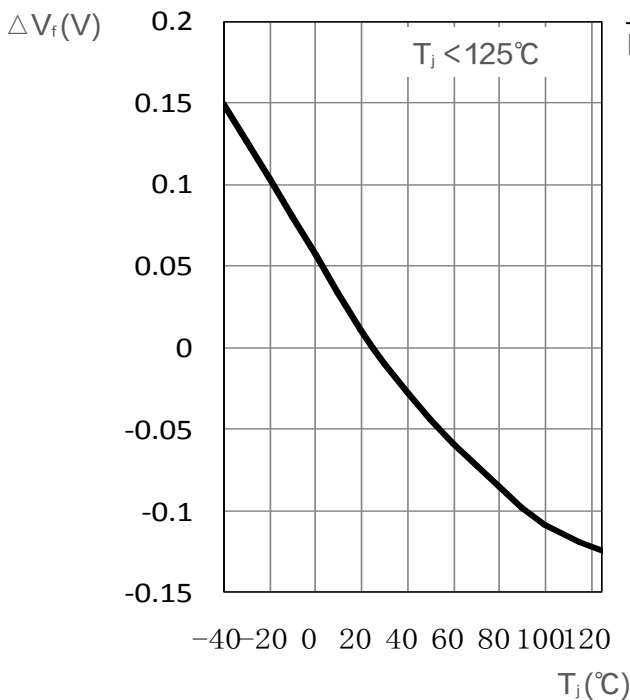
相对正向电压 / Relative Forward Voltage \Delta V_f = V_f - V_f(25^\circ C) = f(T_j); I_f = 50 mA
