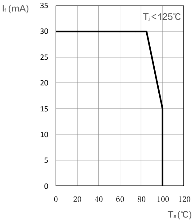
环境温度与正向电流 Ambient Temperature vs. Forward Current I_f = f(T_a)
