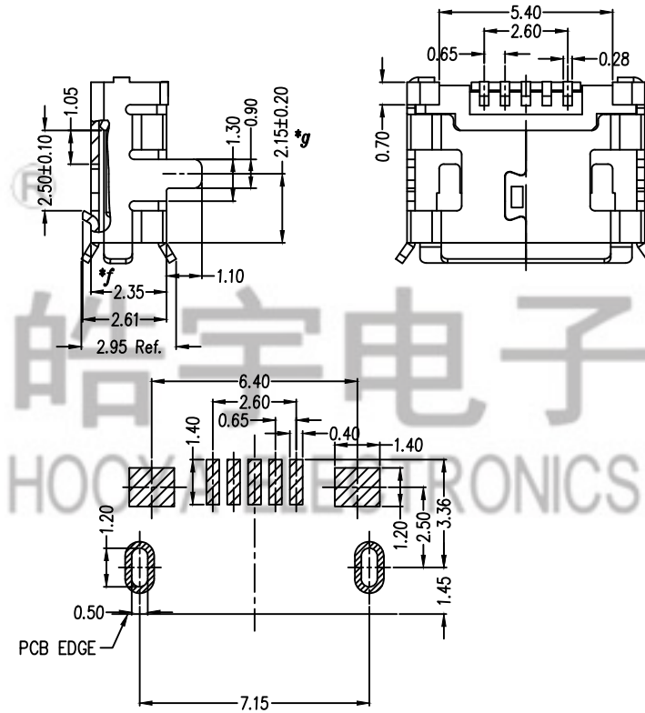
RECOMMENDED PCB LAYOUT PCB图仅供参考
