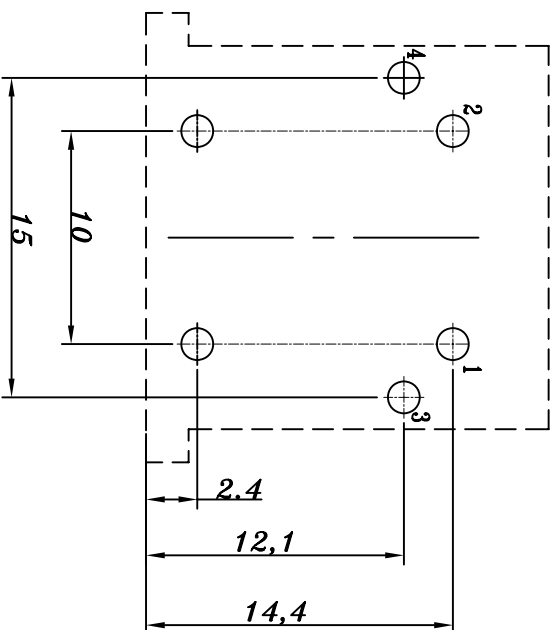
PCB LAYOUT
