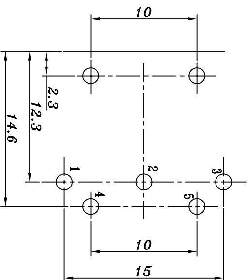
PCB LAYOUT
