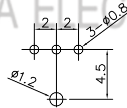
P. C. B LAYOUT
