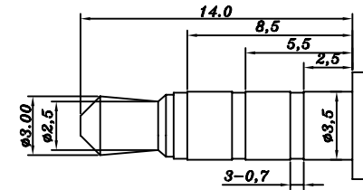
(ø3.50mm 4 POLE PLUG DETAIL DRAWING)
