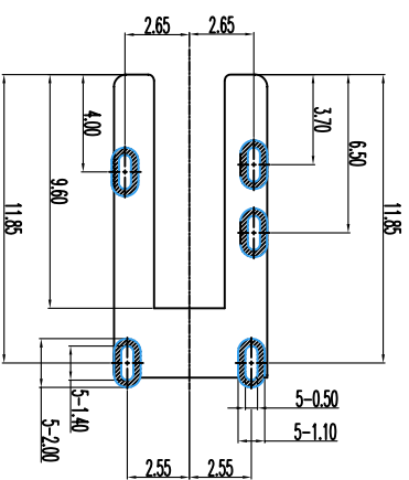
RECOMMEND FPC LAYOUT TOLERANCE: ±0.05
