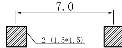
PCB LAND PATTERN
